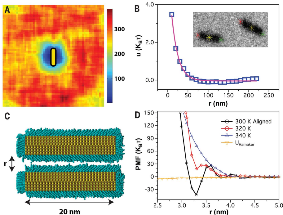
Fig. 5. Experimental and computational methods to obtain potential of mean force. (A) Color-coded counts of the total number of rods in the 2D plane pixels obtained by the real-time monitoring of nanorod behavior in liquid by TEM (132). (B) Experimental PMF for Au nanorods (inset) obtained by TEM imaging in liquid cells. (C) CdS 4-nm-by-20-nm faceted nanorods coated with alkyl thiol molecules and (D) their simulated PMFs at the temperatures indicated in n -hexane, where r is the distance between the opposing crystal facets (114).
